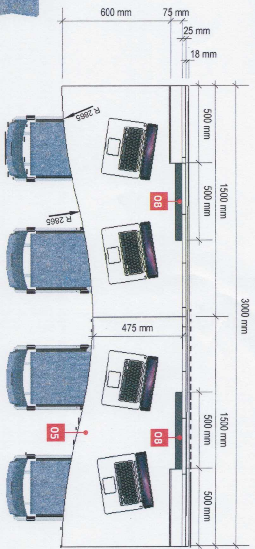
TOP VIEW
